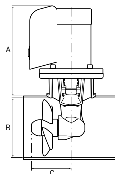
Single Propeller
