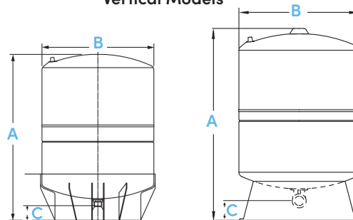
Vertical Models
