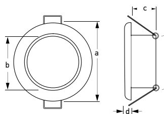
EuroLED 75 RGB/W
