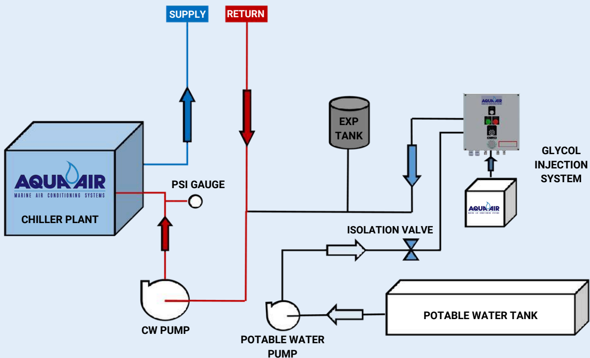
GLYCOL INJECTION SYSTEM™ PLUMBING DIAGRAM
