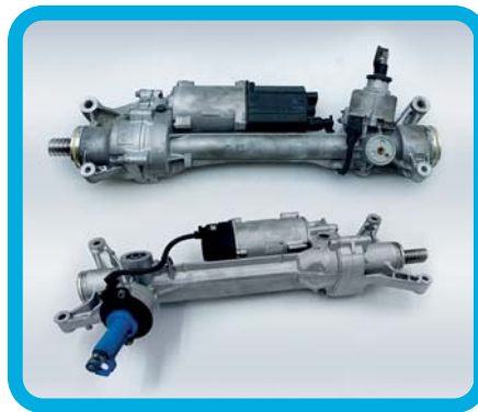
Mercedes-Benz W205 C-Class
