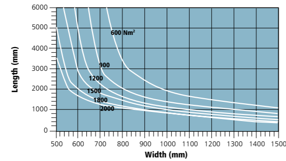
ALVECOLAR 20 mm 5 WALLS X
