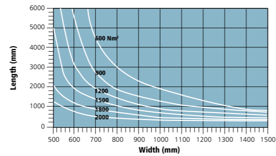
ALVECOLAR 16 mm 5 WALLS X / 10 WALLS X
