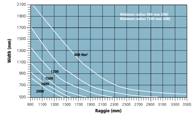
ALVECOLAR 6mm 2 WALLS
