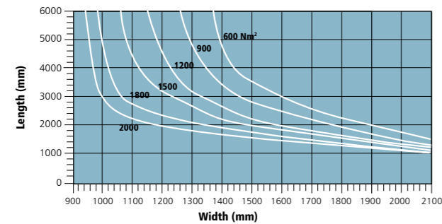
ALVECOLAR 32/35 mm 10 WALLS X
