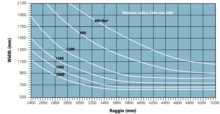
ALVECOLAR 20mm 5 WALLS X
