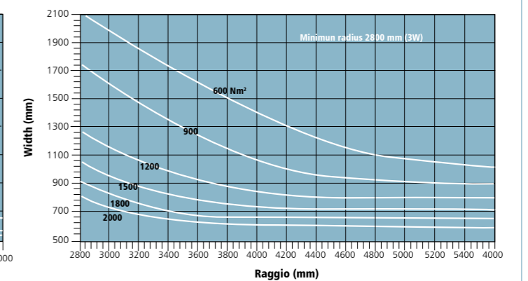
ALVECOLAR 16mm 5 WALLS X
