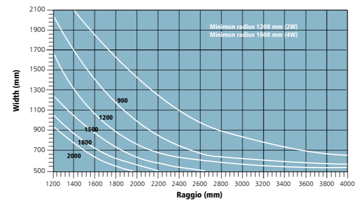
ALVECOLAR 8mm 2 WALLS
