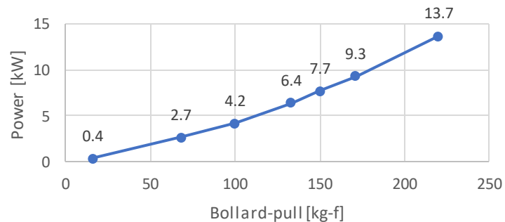
Bollard-pull vs. input power
