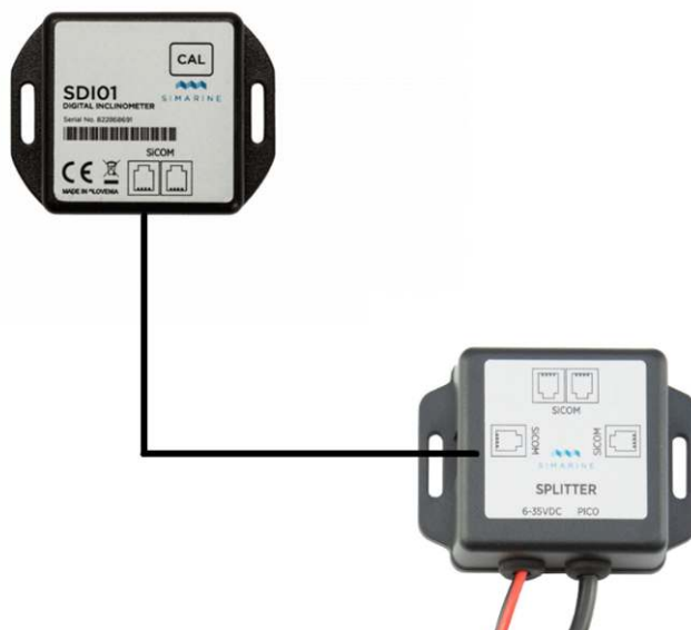
STANDARD WIRING – DIRECTLY TO THE SPLITTER
