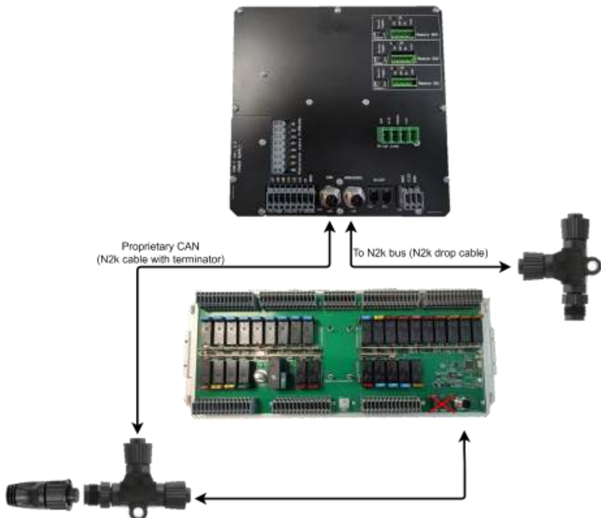
Figure 14: Connecting the panel to the distribution unit and NMEA2000 network.
