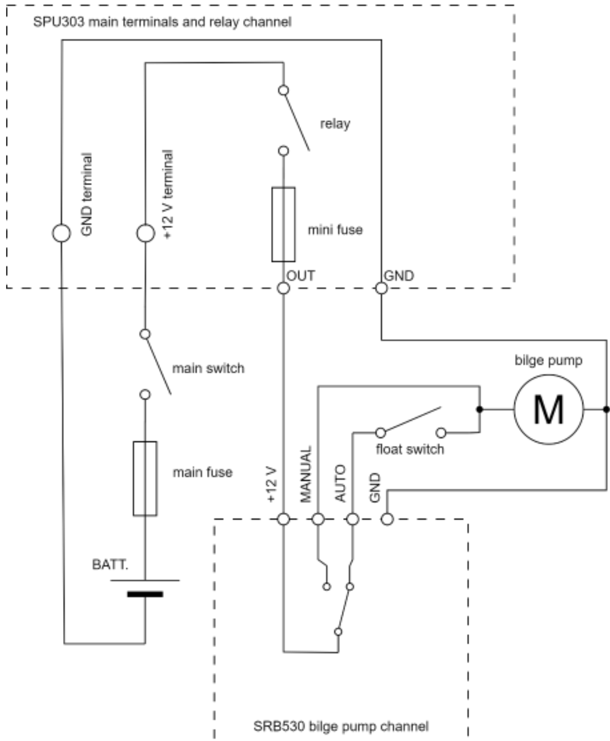
Figure 7: Three-way bilge pump switch schematic.
