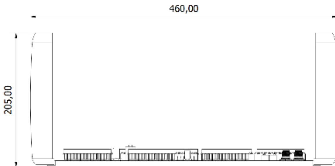
Figure 25: SPU303 dimension with open covers.
