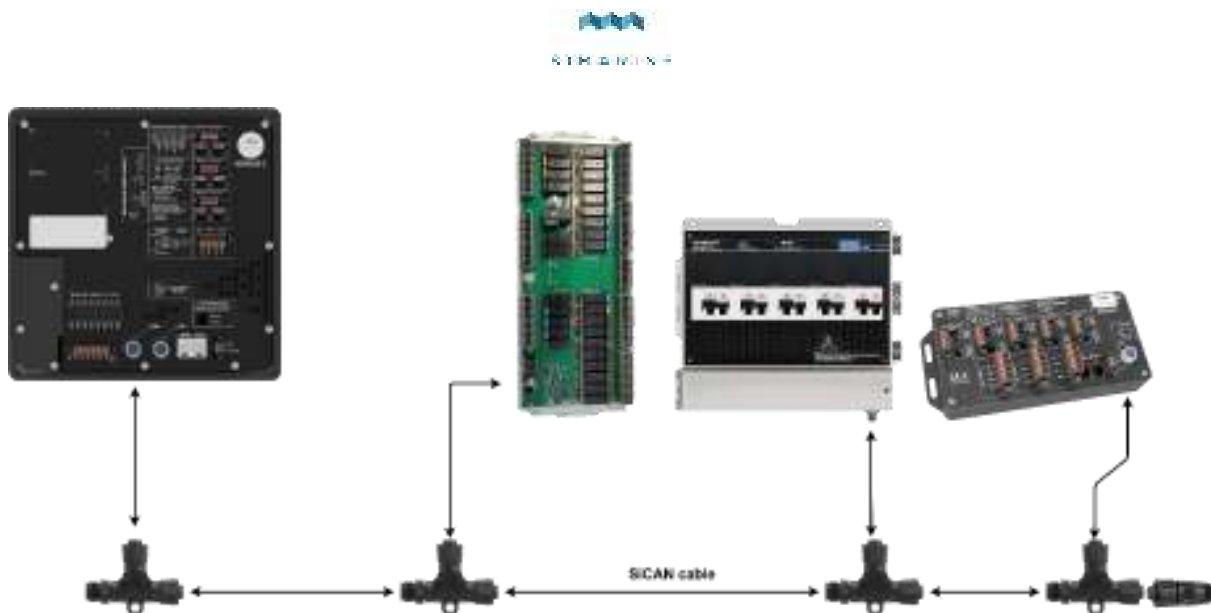
Figure 15: Example of connecting other SiCAN devices to the control panel.
