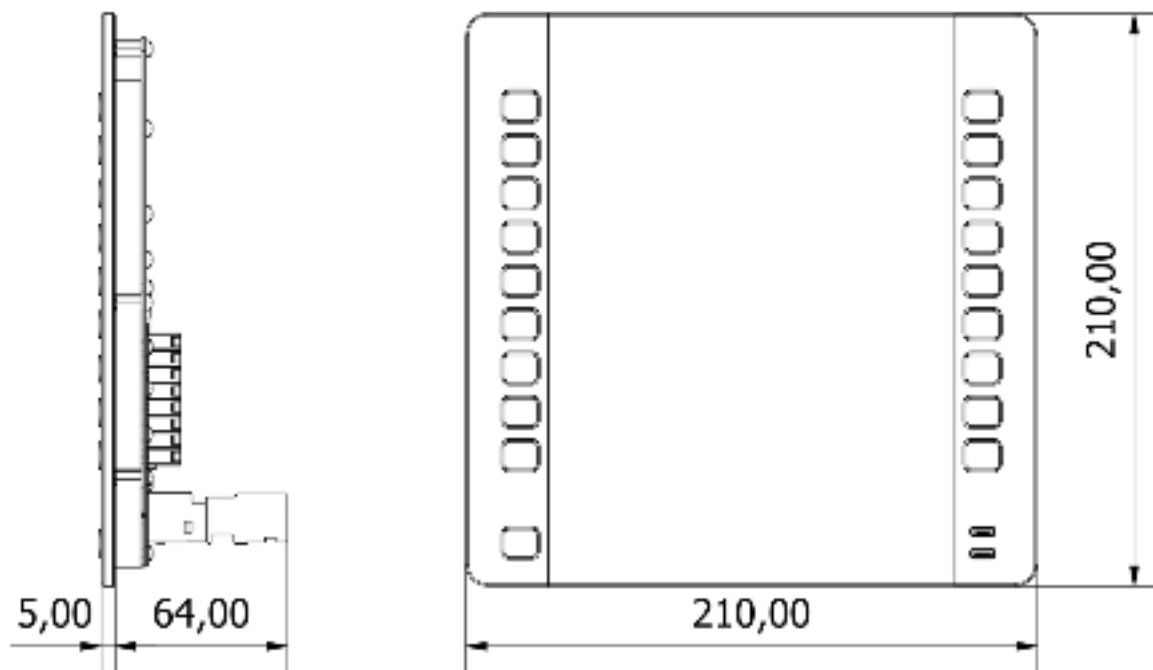
Figure 23: Nereide 2 general dimensions.
