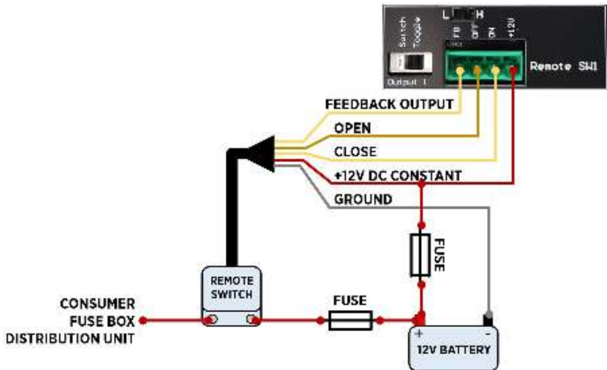
Figure 11: Toggle signal type of remote switch.
