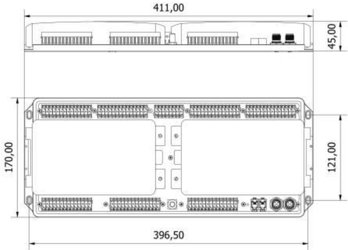
Figure 24: SPU303 DC Distribution Unit general dimensions.
