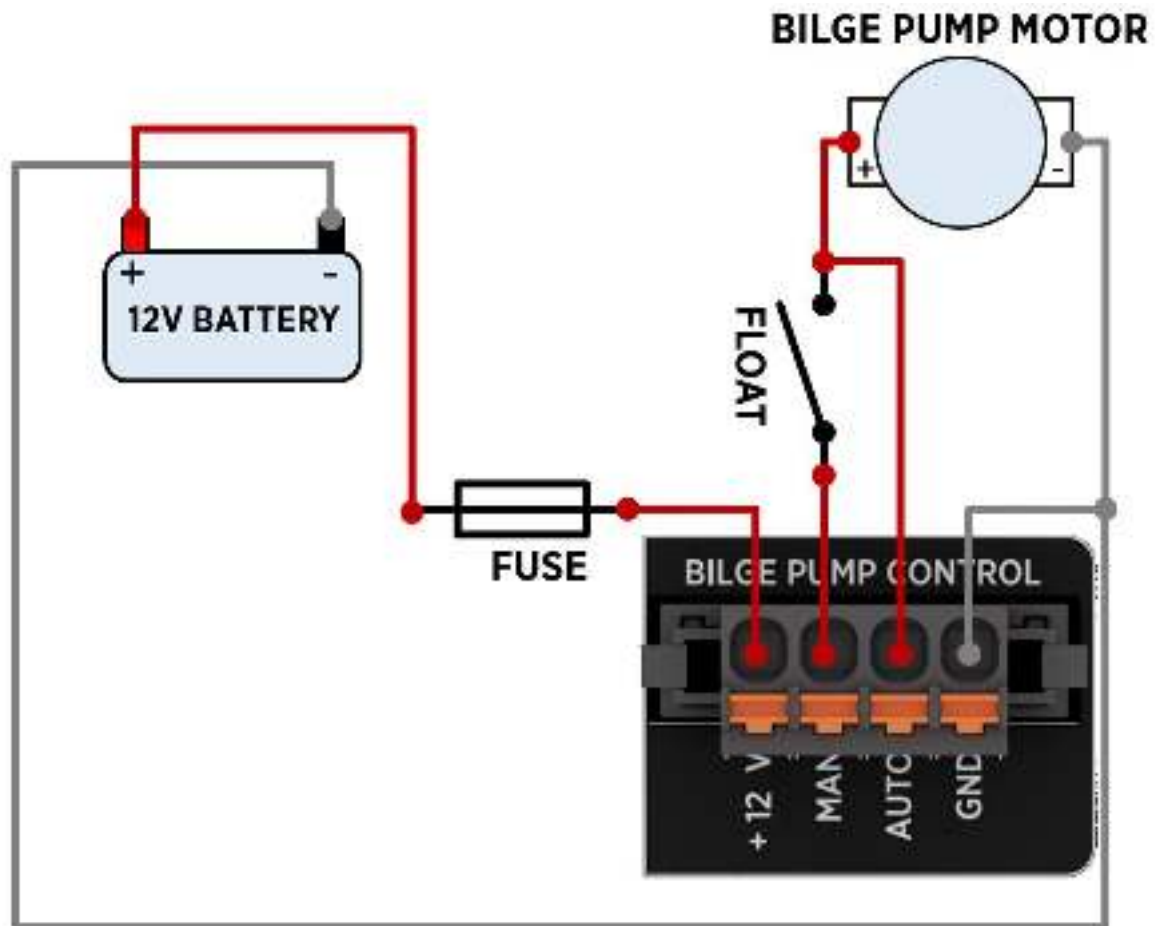
Figure 4: Connecting a bilge pump.
