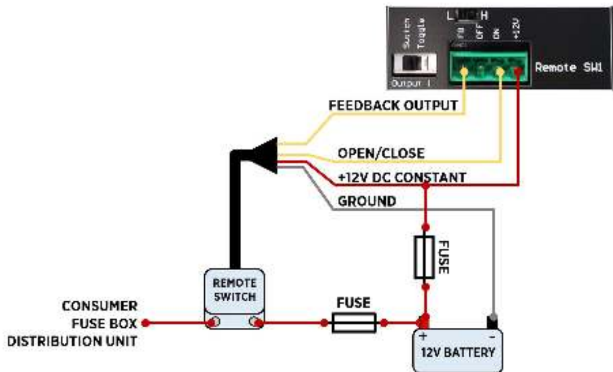
Figure 12: Switch signal type of remote switch.
