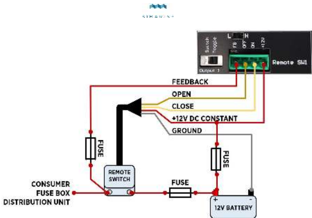
Figure 13: Feedback signal from remote switch output.
