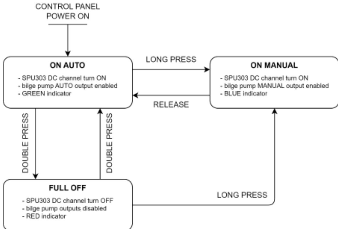
Figure 8: State diagram of three-way bilge pump button mode.
