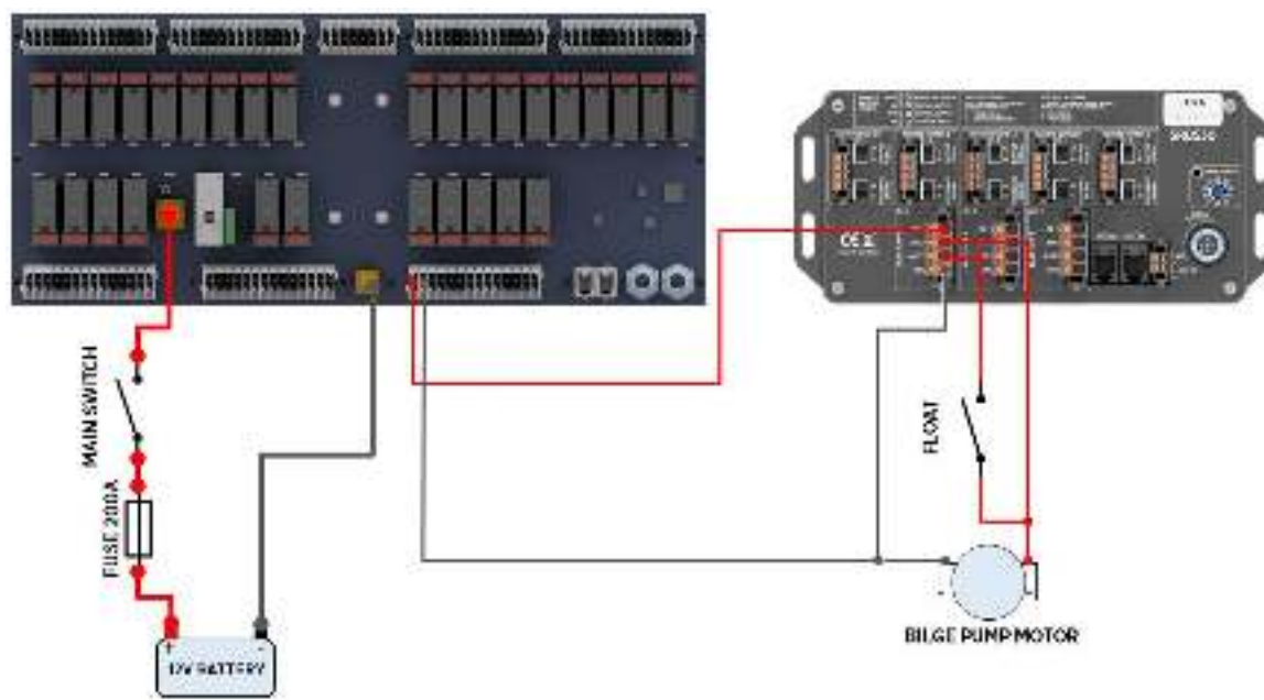
Figure 6: Example of three-way bilge pump switch mode implementation.
