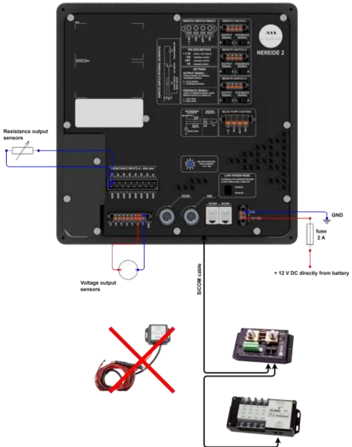
Figure 3: Control panel connections diagram.
