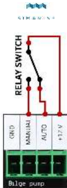
Figure 5: Internal schematics of the bilge pump connector.
