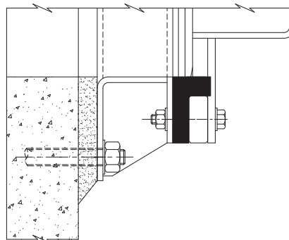
BOTTOM SEALING ARRANGEMENT
