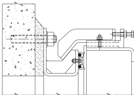
TOP SEALING ARRANGEMENT
