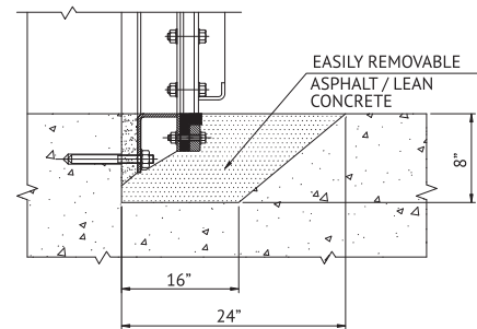
FLUSH BOTTOM CLOSURE CIVIL DETAILS
