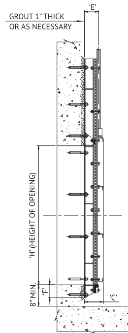
SIDE VIEW
