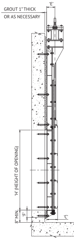
SIDE VIEW
