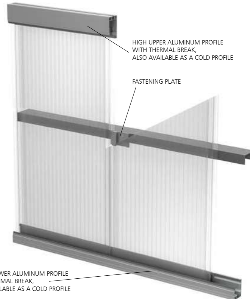
LOWER PROFILE DETAIL OF FASTENING, ALSO AVAILABLE WITH THERMALLY BROKEN PROFILES
