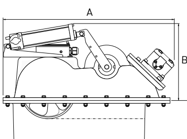
Hydraulic Retractable Thrusters Diam. 185 mm
