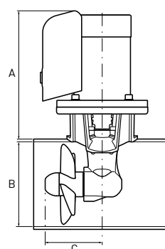
Single Propeller
