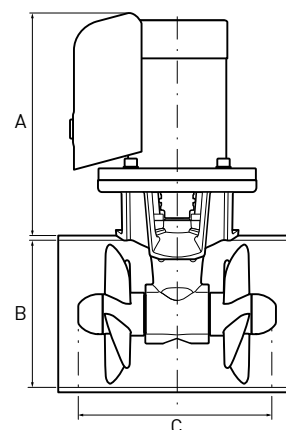
Double Propeller
