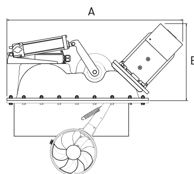
DC Retractable Thrusters Diam. 185 mm
