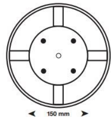
BASE Fixing Holes 14 mm at 80 mm centres to suit fixings illustrated opposite
