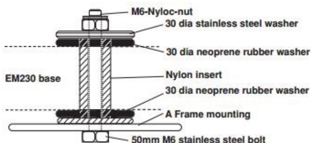
BASE Fixing Holes 14 mm at 80 mm centres to suit fixings illustrated opposite
