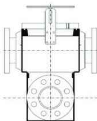
2 INLET - 1 OUTLET
