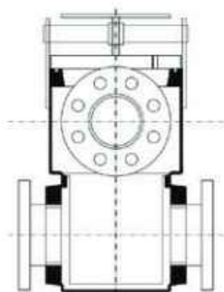
1 INLET - 2 OUTLET
