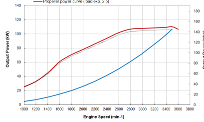
4LV170 Output Power curve
