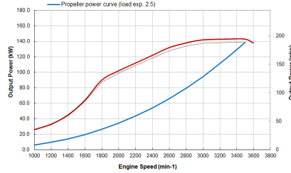
4LV195 Output Power curve
