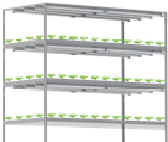
Grow rack setup vegetative growth 8 lamps per canopy layer in 4 daisy-chain lines with reduced cabling PPFD 435 \mu mol/sm 2
