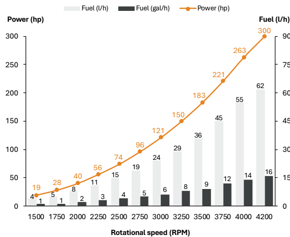
Propeller Chart
