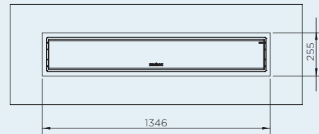
MINIMUM CAVITY OPTION 2 2300/3400W
