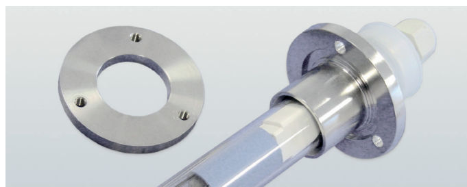
TRS 23 with screw-on flange and counter ring made of stainless steel
