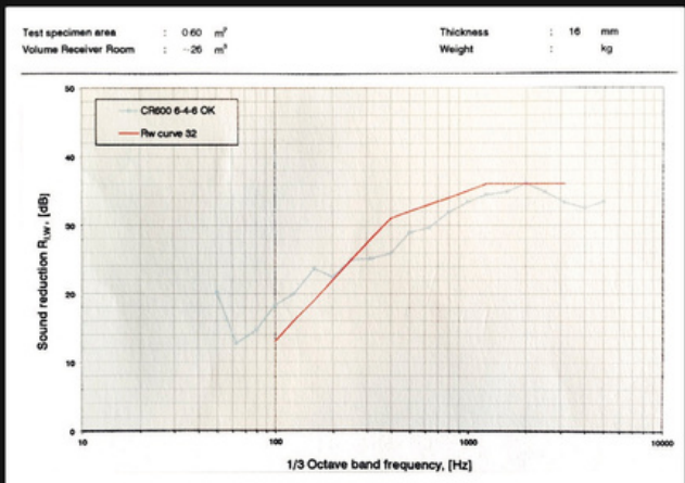
Example test result CR 600 6-4-6 Okoume
