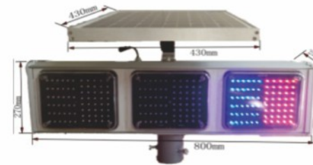
Size:800X252X270mm 型号(model):LZL-SL-13
