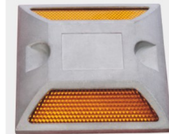
型号(model):LZL-DD-03 材料(material):塑料(plastic); PC反光片(PCreflective sheeting) 规格(specification):单面或双面反光 (single or double-side) 尺寸(size):100×100×20mm
