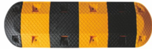
LZL-PSH-01 Middle Size: 250x350x50mm End Cap Size: 170X350X50mm weight: 5.4kg
