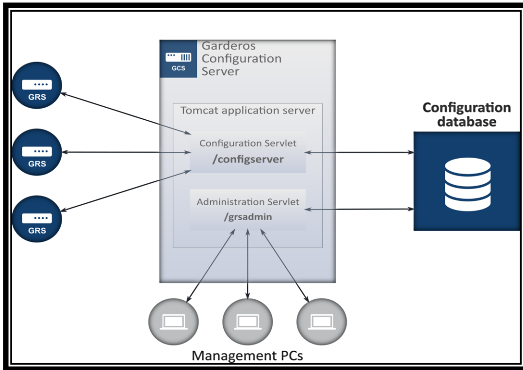
Fig. 1: Basic architecture
