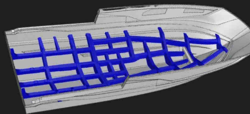
Structural Scantlings
